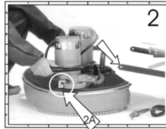
Brush Assembly Mount
